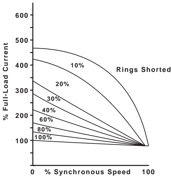
Figure 23. Wound rotor induction motor characteristics
