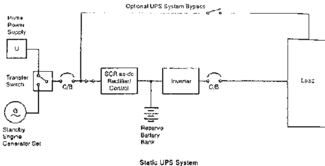
Static UPS System
